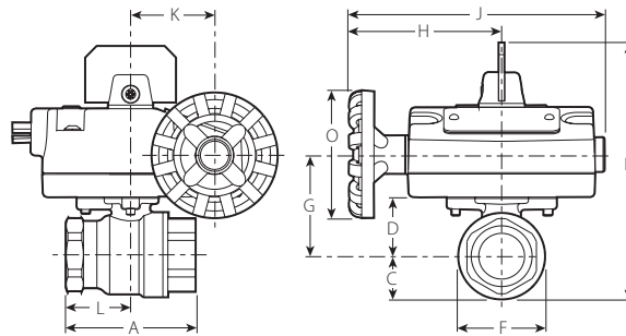
THREADED x THREADED TYPICAL OF ALL SIZES
